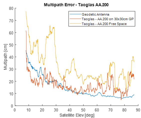
Fig. 8. Standard deviation of the multipath error for GPS L1-C/A signal. Ground plane effect on Taoglas AA.200.
